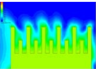
Figure 13: Analysis results in a temperature cut plot, showing the front view, as obtained for heat sink No. 2
