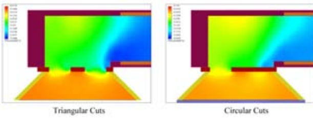
Figure 18: Pressure cut plots for each design. Both designs have similar pressure profiles.
