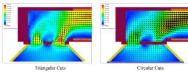
Figure 19: Velocity cut plots with velocity vectors for each design. Both designs have similar velocity profiles at the suction head.
