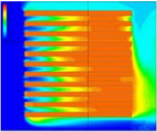
Figure 10: Temperature cut plot, showing the topview, as obtained for heat sink No. 1
