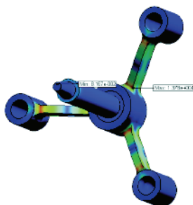
spenningsanalyse
